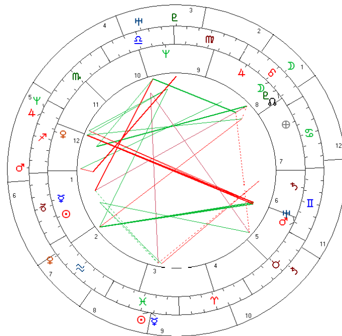
fig. 2. Transits 08/03/1971
