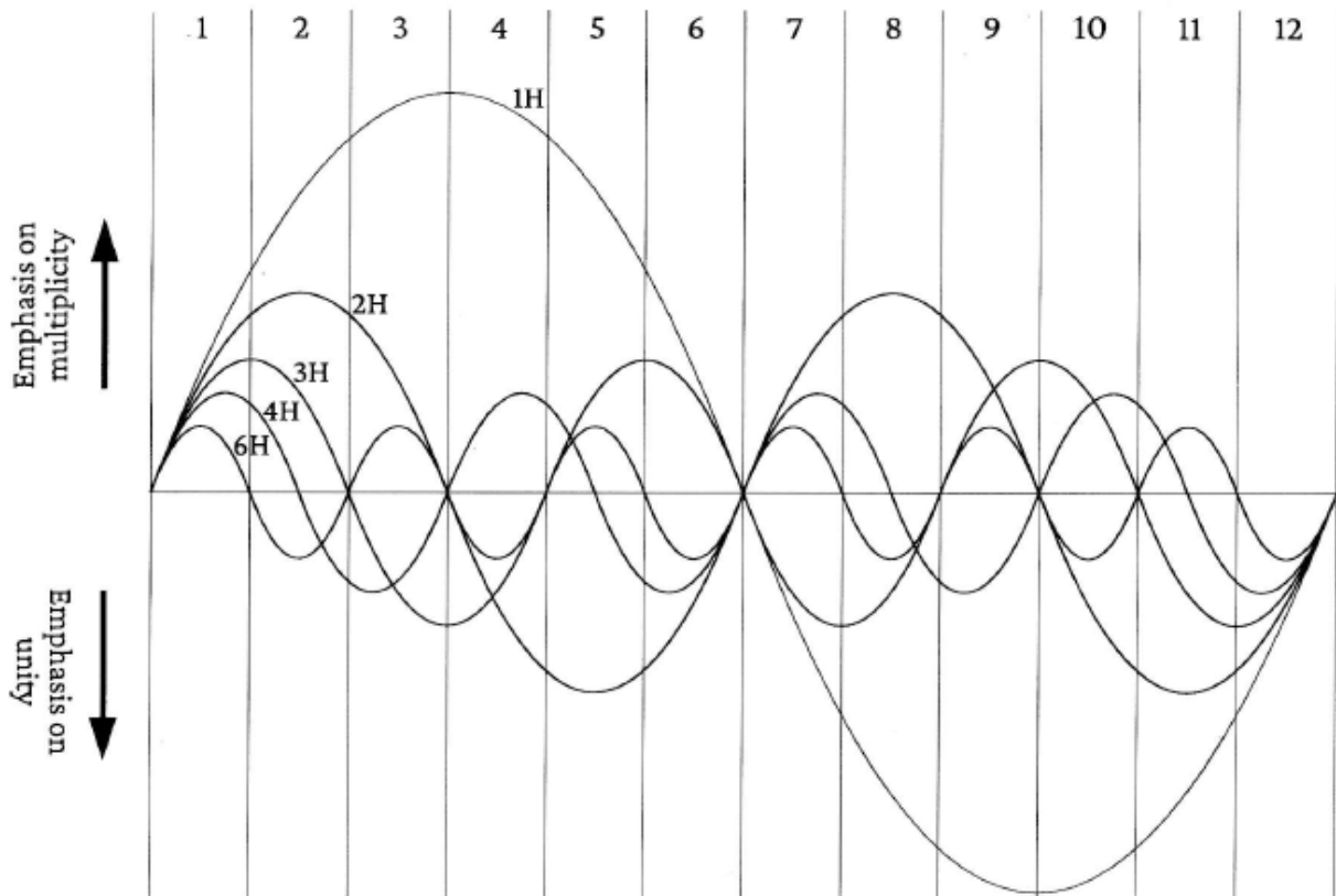
Figure 4.4 The harmonic basis of the twelve-fold division
